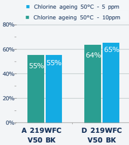
Tensile Strength Retention from DAM (%)
