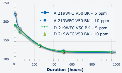
Tensile Strength from DAM (MPa)
